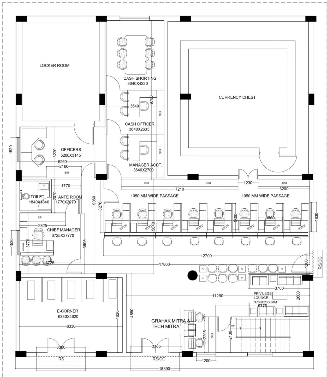
GROUND FLOOR SCHEMATIC PLAN
