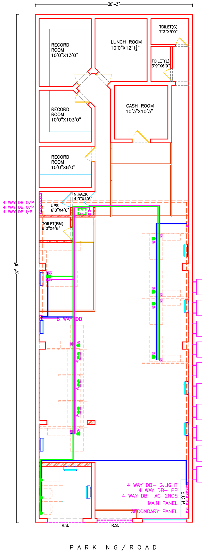
LAYOUT PLAN - G.F.
