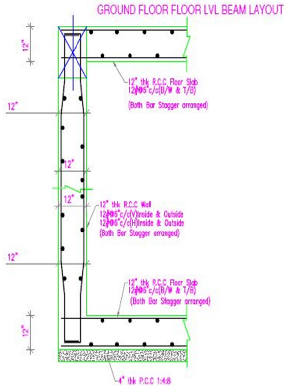
TYP SECTION OF RCC WALL AND FLOOR / ROOF SLAB
