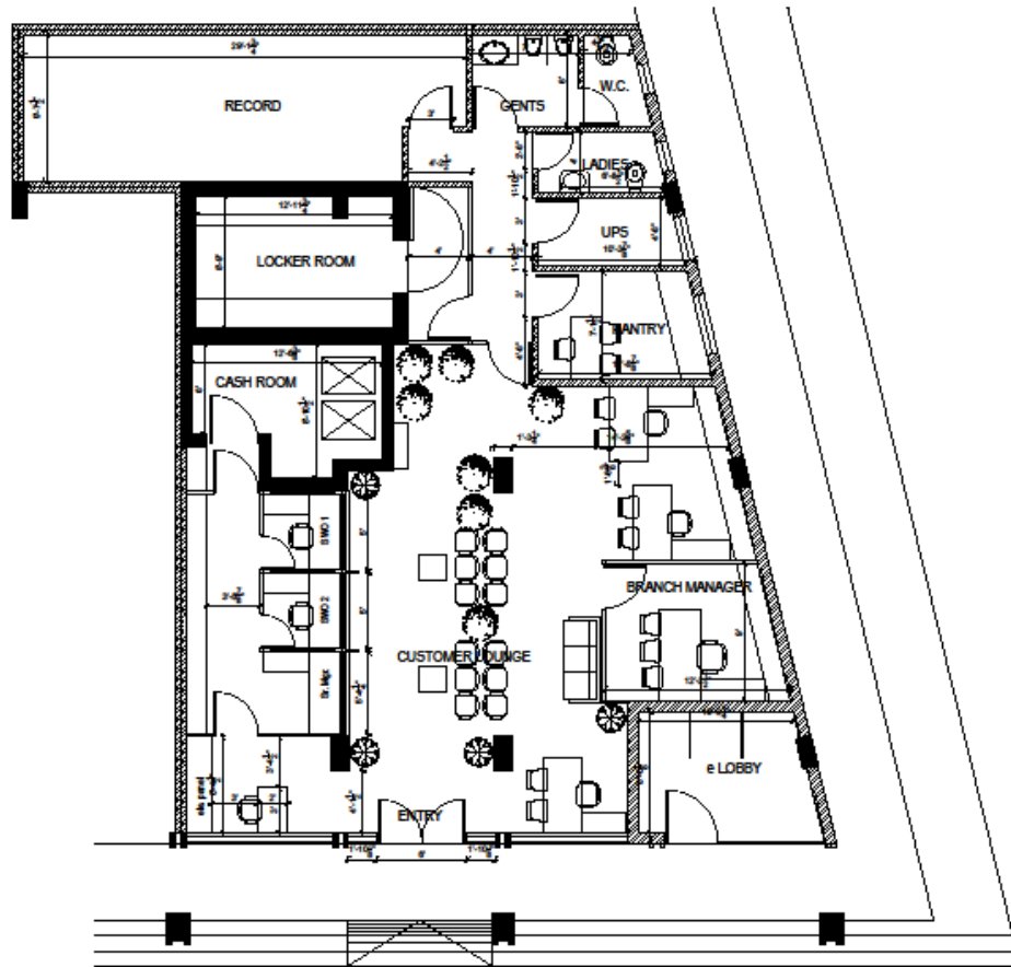
PROJECT MEHTAPURA BRANCH . SBI . HIMMATNAGAR. GROUND FLOOR PLAN
