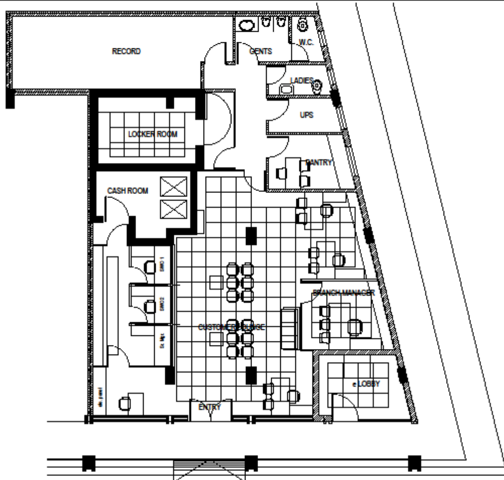
PROJECT MEHTAPURA BRANCH . HIMMATNAGAR . SBI . RBO II GROUND FLOOR PLAN - FALSE CEILING
