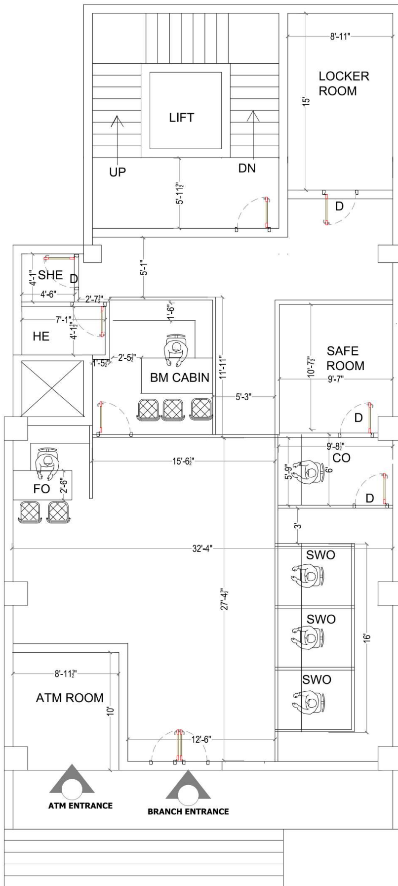
GROUND FLOOR SURYAPET TOWN BRANCH
