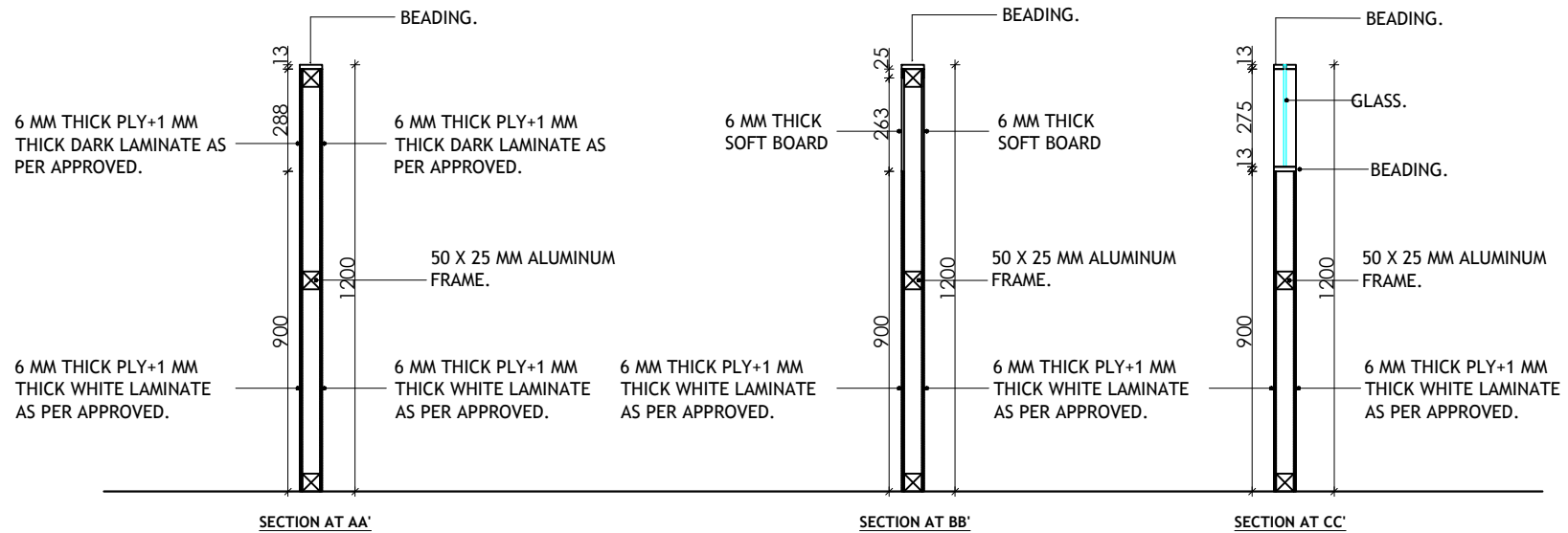
SALES AREA PARTITION DETAIL
