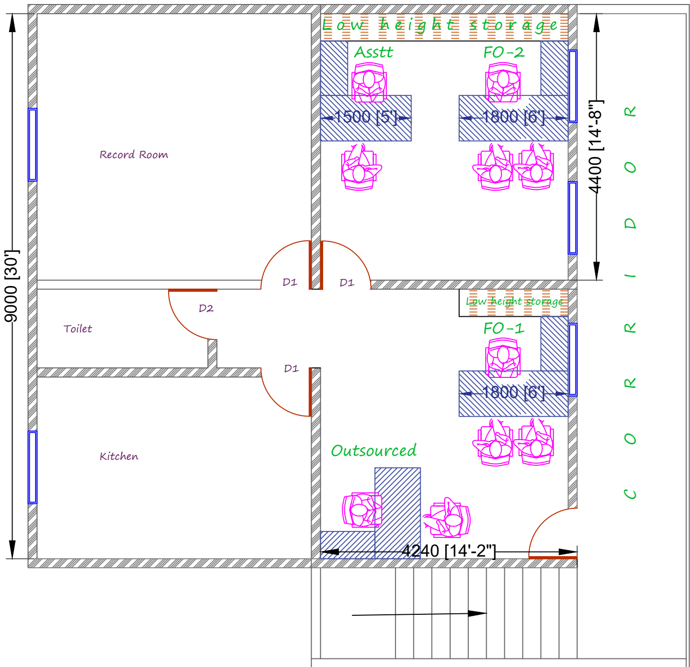
PLAN OF KANGPOKPI BRANCH SECOND FLOOR
