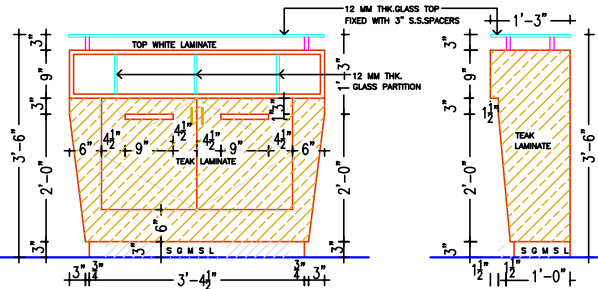
FRONT ELEVATION
