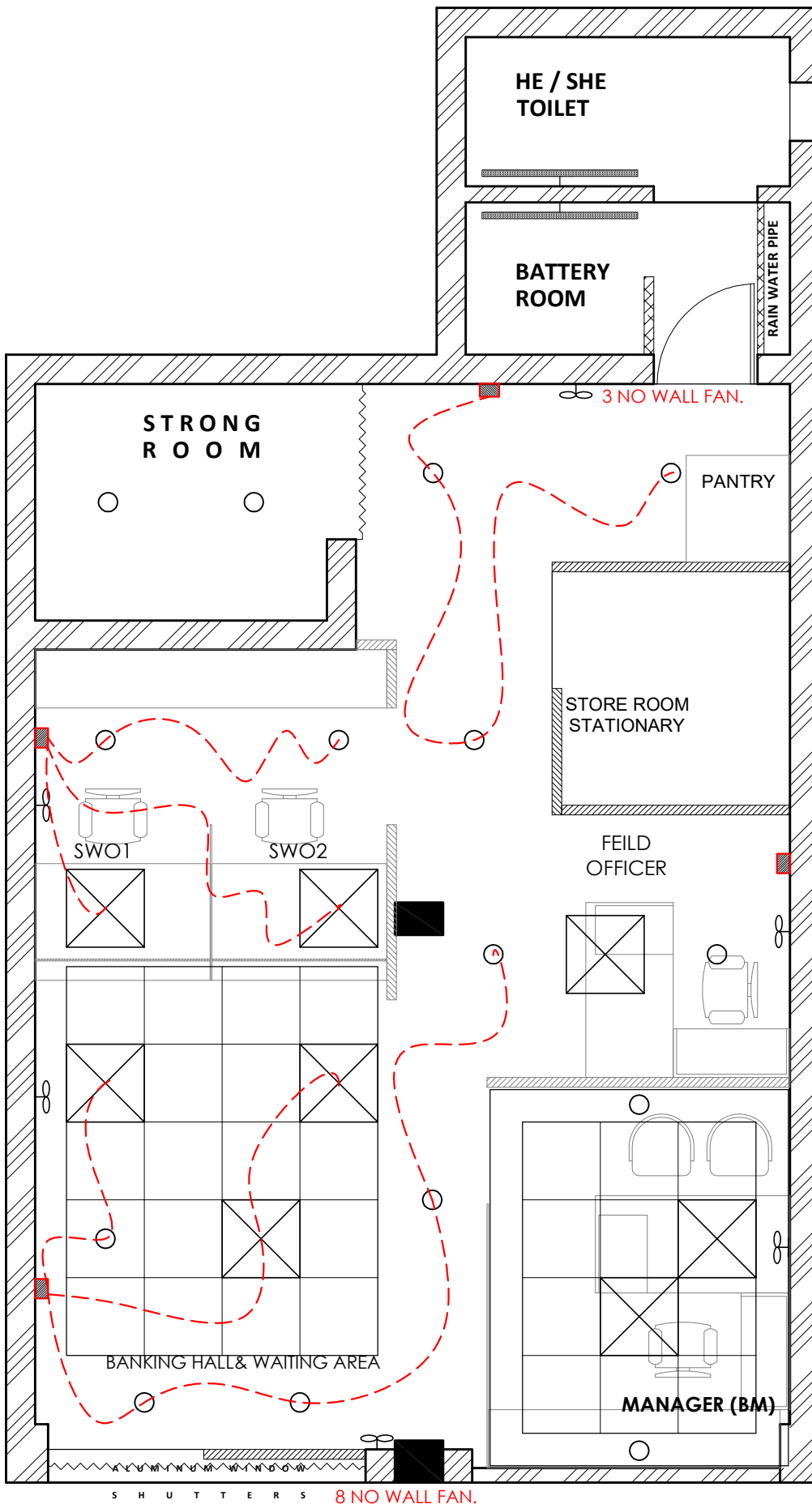
ELECTRICAL AND LIGHTING LAYOUT PLAN WITH POINT WIRING AND SWITCHBOARD
